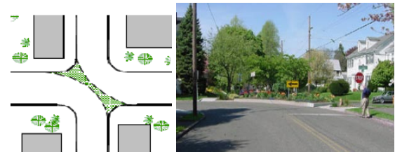
13 - Diverters
